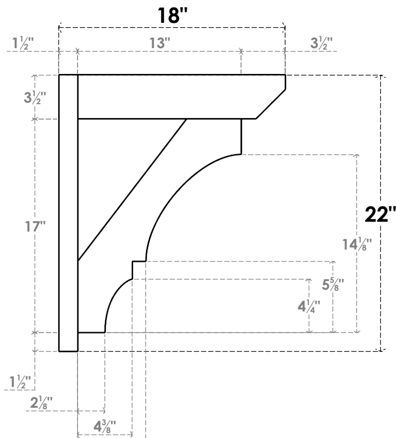
SIDE PROFILE
